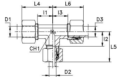
Typ: 1045...4 Ring B4
